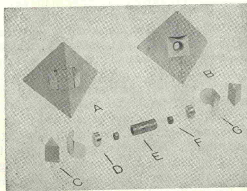
FIG. 1. Pyrophyllite sample-holder and assembly.
